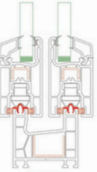
MONTAJ ÇİZİMİ ASSEMBLY DRAWING
