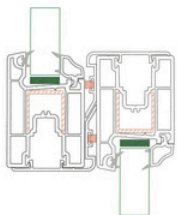
MONTAJ ÇİZİMİ ASSEMBLY DRAWING
