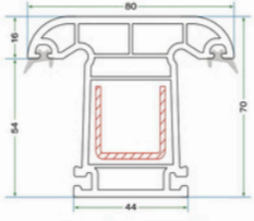
KRS 002 70'LIK ORTA KAYIT PROFİLİ KRS 002 70 MULLION PROFILE
