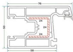
KPS 6202 PERVAZLI SÜRME KANAT PROFİLİ KPS 6202 SLIDING SASH PROFILE WITH BORDER
