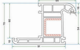
KRS 005 70'LIK PERVAZLI KASA PROFİLİ KRS 005 70 FRAME PROFILE WITH BORDER
