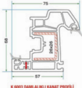
K 6003 DAMLALIKLI KANAT PROFİLİ K 6003 DROPPER SASH PROFILE
