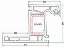
K 6019 PERVAZLI KASA PROFİLİ K 6019 FRAME PROFILE WITH BORDER
