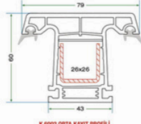
K 6002 ORTA KAYIT PROFİLİ K 6002 MULLION PROFILE
