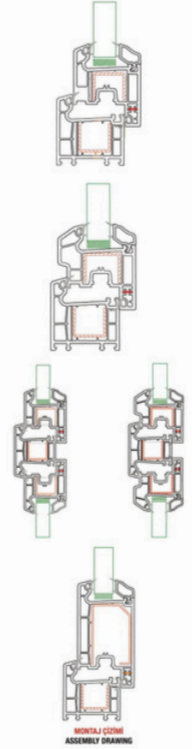
ORTA KAYIT DESTEK SAÇI K 6001 MULLION STEEL REINFORCEMENT
