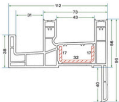
KPS 6201 PERVAZLI SÜRME SİNEKLİK KASA PROFİLİ KPS 6201 FLY SCREEN SLIDING FRAME PROFILE WITH BORDER
