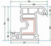
KRS 003 70'LIK DÜZ KANAT PROFİLİ KRS 003 70 FLAT SASH PROFILE
