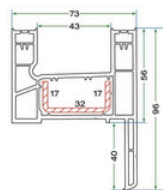
KPS 6207 PERVAZLI SÜRME KASA PROFİLİ KPS 6207 SLIDING FRAME PROFILE WITH BORDER
