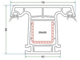
K 6002 ORTA KAYIT PROFİLİ K 6002 MULLION PROFILE
