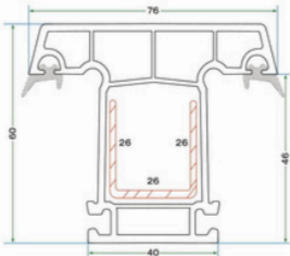
KYS 6002 ORTA KAYIT PROFİLİ KYS 6002 MULLION PROFILE
