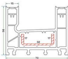
KPS 6208 ÇİFTLİ SÜRME KASA KPS 6208 DOUBLE RAIL SLIDING FRAME PROFILE
