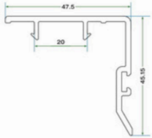
KES 003 KİLİTLEME PROFİLİ KES 003 LOCKING PROFILE
