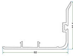
KSS 6104 KİLİTLEME PROFİLİ KSS 6104 LOCKING PROFILE
