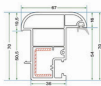
KRS 009 70'LIK OVAL HAREKETLİ ORTA KAYIT PROFİLİ KRS 009 OVAL MOVABLE MULLION PROFILE
