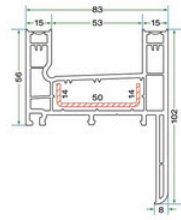
KSS 6103 PERVAZLI 60'LIK SÜRME KASA PROFİLİ KSS 6103 60 SLIDING FRAME PROFILE WITH BORDER
