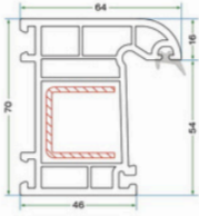
KRS 001 70'LIK KASA PROFİLİ KRS 001 70 FRAME PROFILE
