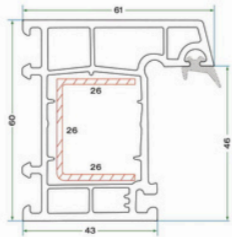
KYS 6001 KASA PROFİLİ KYS 6001 FRAME PROFILE
