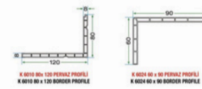
K 6010 80 x 120 PERVAZLI PROFİLİ K 6010 80 x 120 BORDER PROFILE
