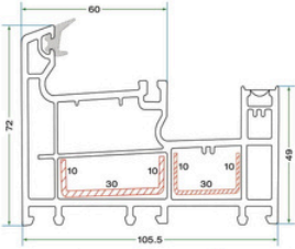
KSS 6105 TEKLİ SÜRME KASA PROFİLİ KSS 6105 SINGLE RAIL SLIDING FRAME PROFILE
