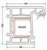
K 6001 KASA PROFİLİ K 6001 FRAME PROFILE
