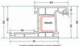
K 6026 GENİŞ PERVAZLI KASA PROFİLİ K 6026 WIDE FRAME PROFILE WITH BORDER
