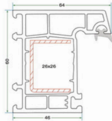
KYS 6004 46'LIK KASA PROFİLİ KYS 6004 46 FRAME PROFILE
